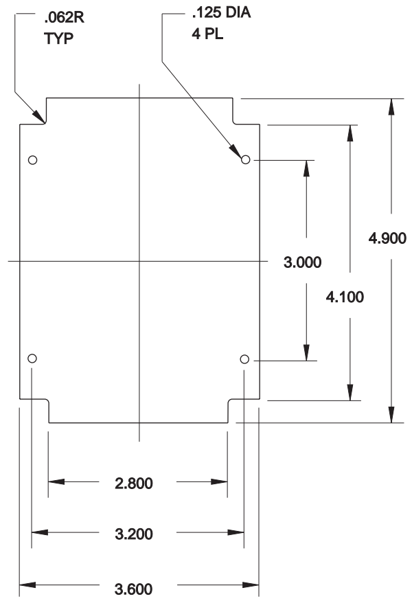
CIRCUIT BOARD REFERENCE DIMENSIONS
