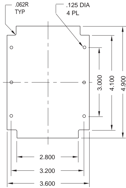
CIRCUIT BOARD REFERENCE DIMENSIONS NOT TO SCALE
